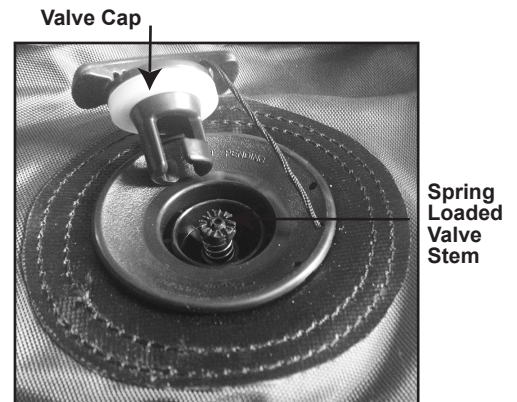
ILLUSTRATION 3 Pro Series Push Button Valve
